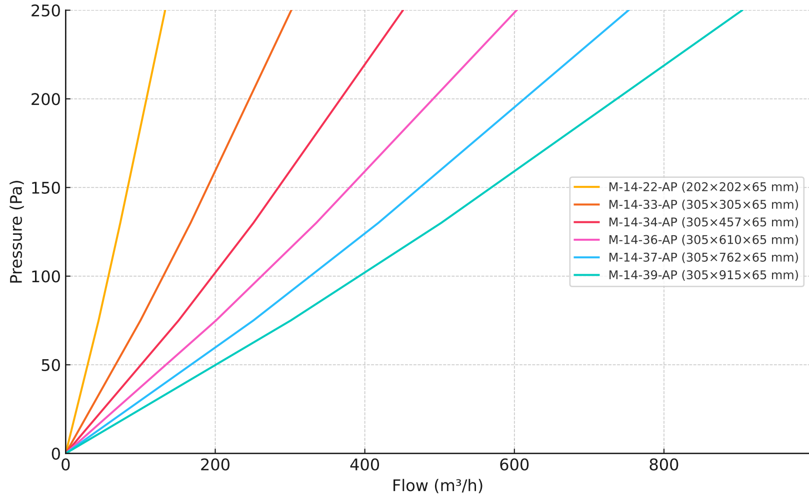
Series M14:3 – Metric Units
