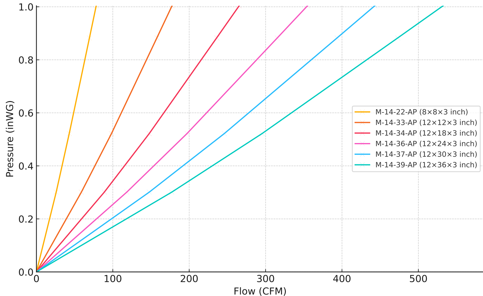
Series M14:3 - Imperial Units
